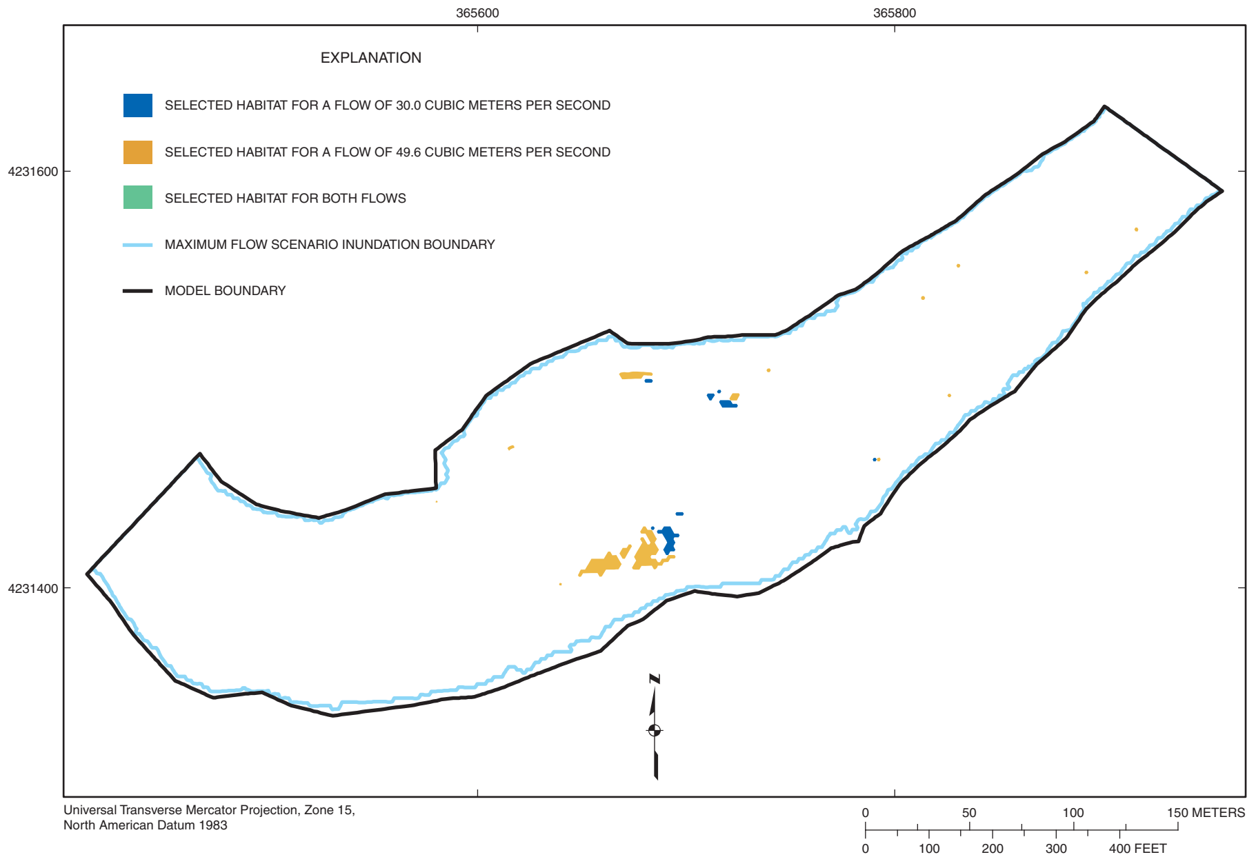
Figure 4-89. Selected habitat area distribution for habitat category 22 (channel catfish) at flows of 30.0 and 49.6 cubic meters per second at Marais des Cygnes River site MDC2.
